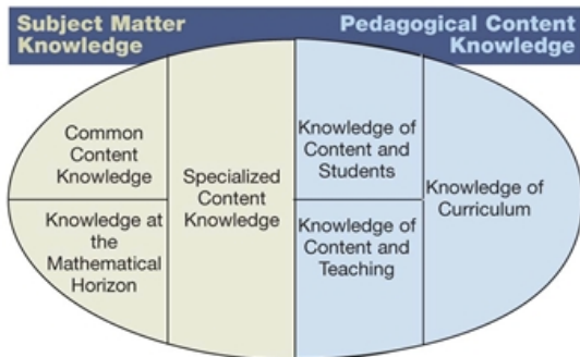
Figure 1. Mathematical Knowledge
